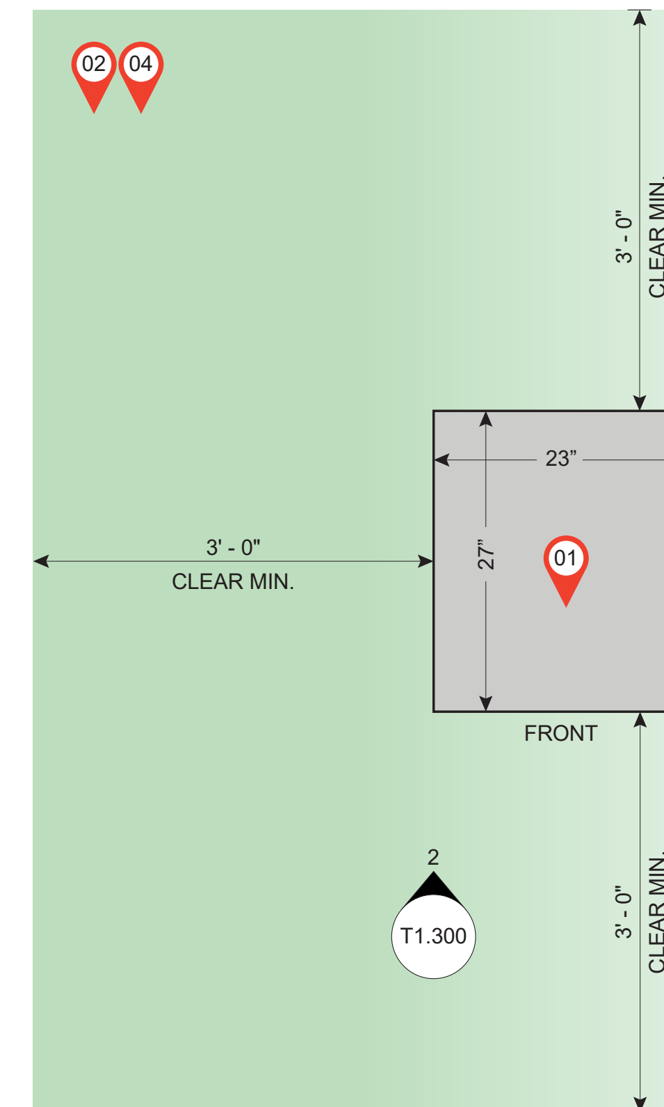
1 AV EQUIPMENT RACK CLEARANCE REQUIREMENTS - PLAN
